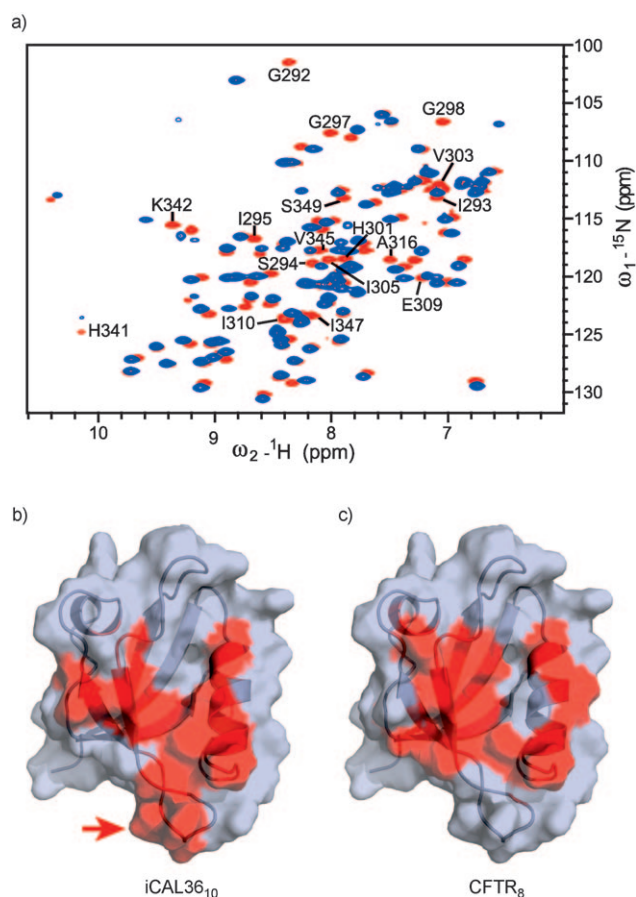
Figure 2. iCAL36 is a competitive inhibitor. a) HSQC spectra of ^{15}N -CALP were determined in the absence (red) and in the presence (blue) of 800 \mu M iCAL36. Cross-peak perturbations are labeled by residue. b, c) Surface representations of the CAL PDZ domain (PDB entry 2DC2) show the overlapping interfaces (red) associated with binding of the iCAL36 decapeptide ANSRWPTSII (b) or with the CFTR C-terminal octamer EEVQDTRL (c). [18] The binding surface of the iCAL36 10 peptide extends beyond that of CFTR 8 (b, arrow).
